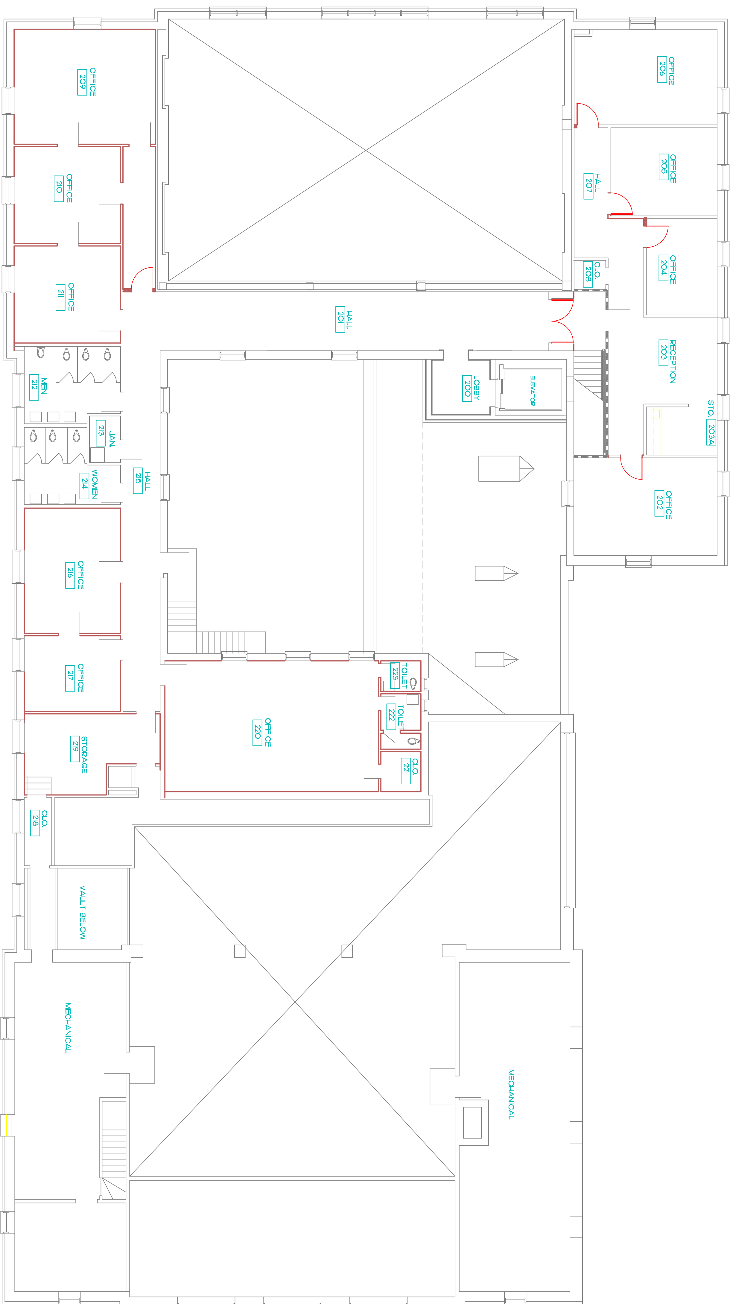
1 UPPER LEVEL FLOOR PLAN A30 1/8" = 1'-0"
